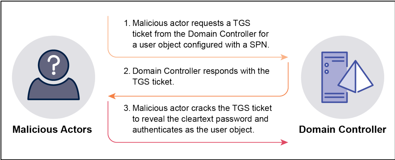
Figure 1: Overview of Kerberoasting
