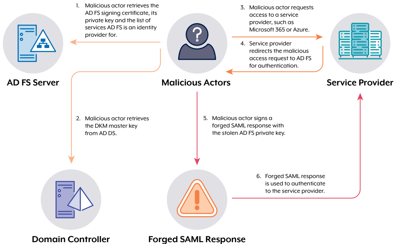
Figure 7. Overview of a Golden SAML
