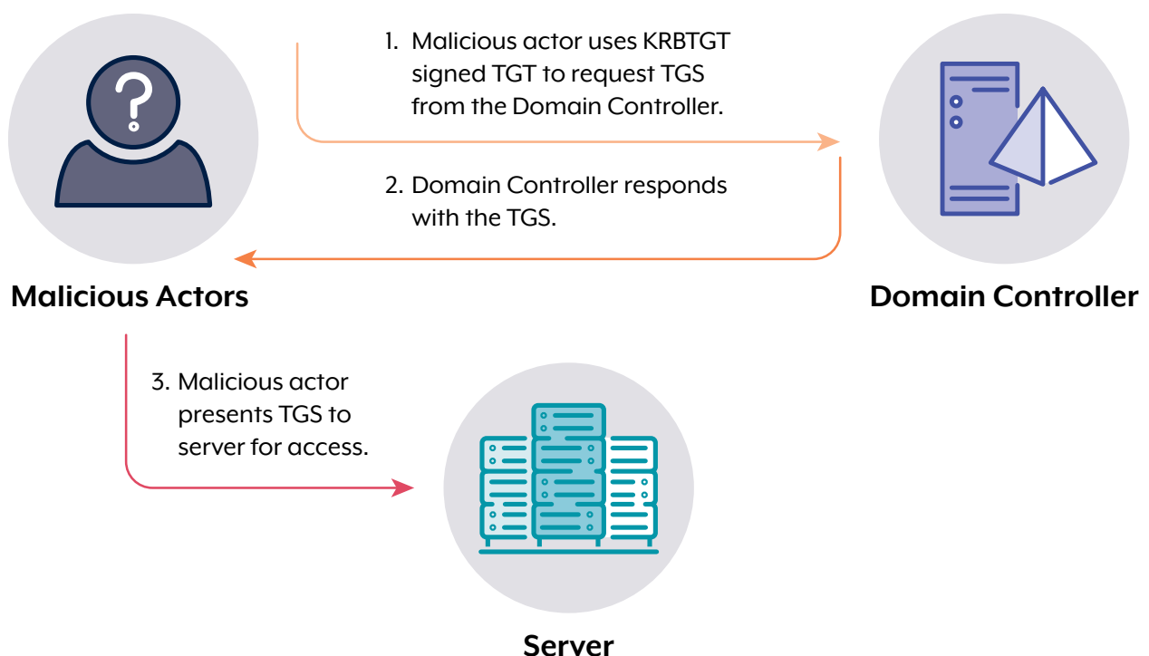
Figure 5. Overview of a Golden Ticket
