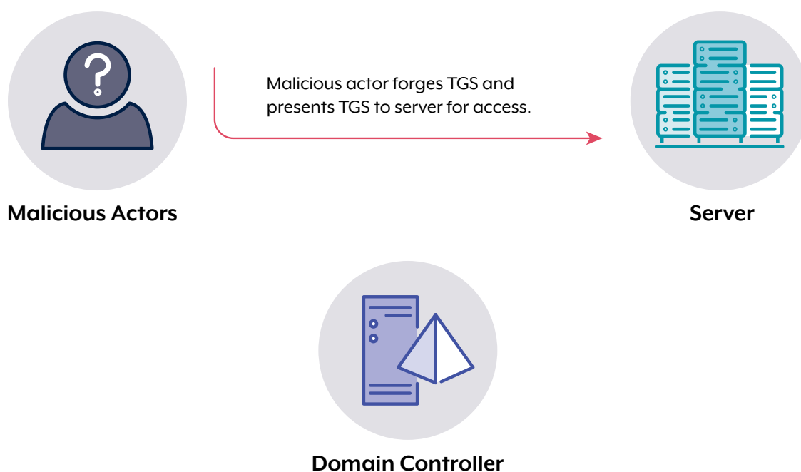
Figure 6. Overview of a Silver Ticket
