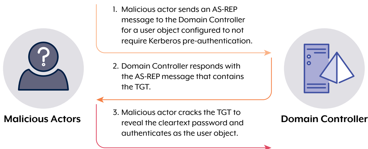
Figure 2. Overview of AS-REP Roasting
