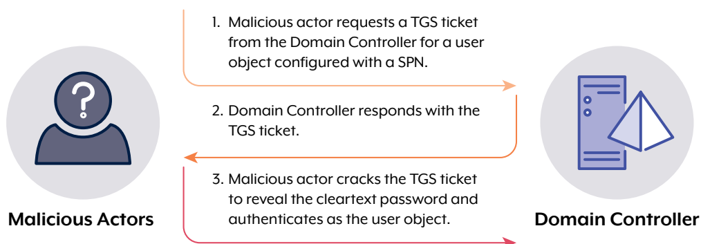
Figure 1. Overview of Kerberoasting
