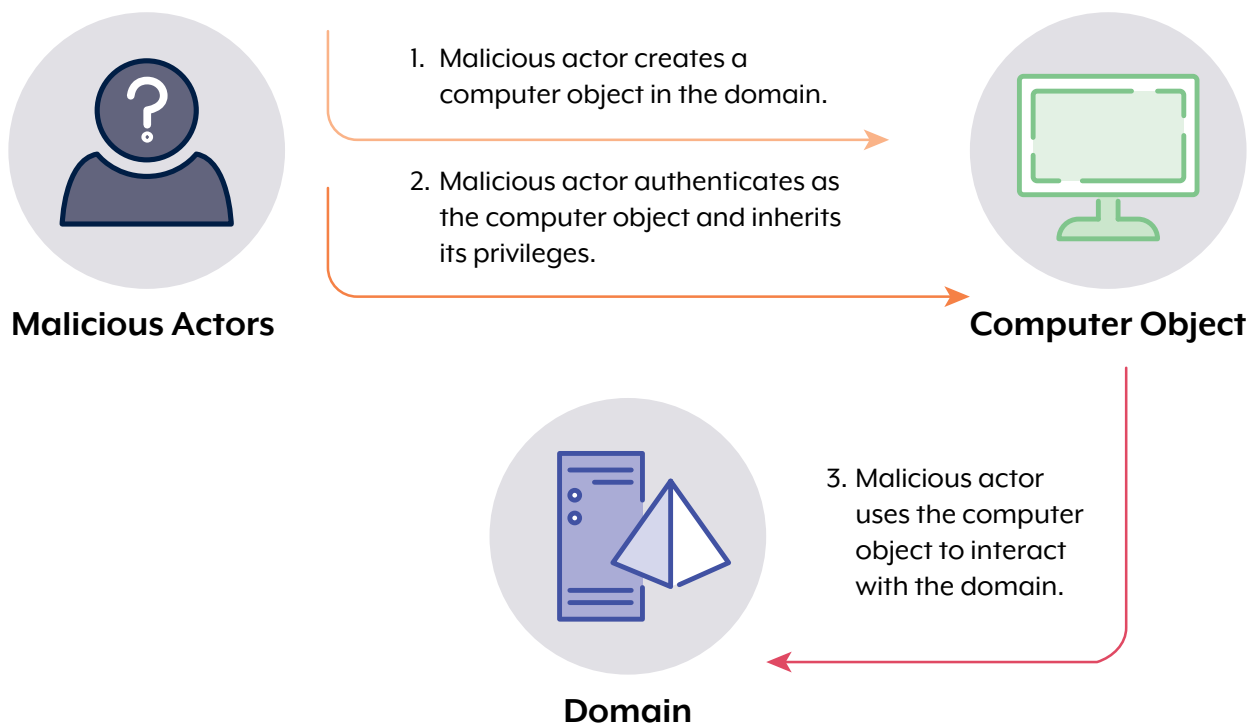
Figure 3. Overview of a MachineAccountQuota compromise
