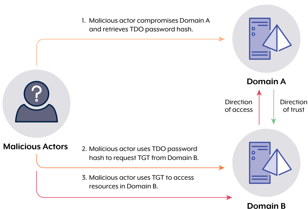
Figure 9. Overview of one-way domain trust bypass
